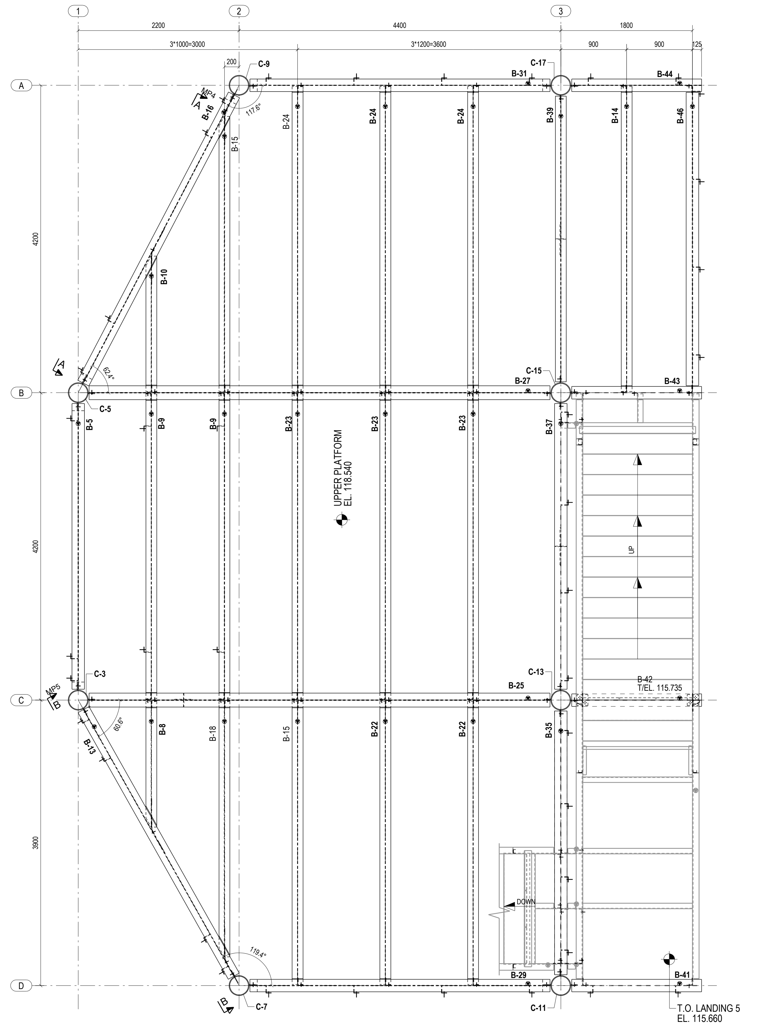
TOWER UPPER PLATFORM FRAMING PLAN
