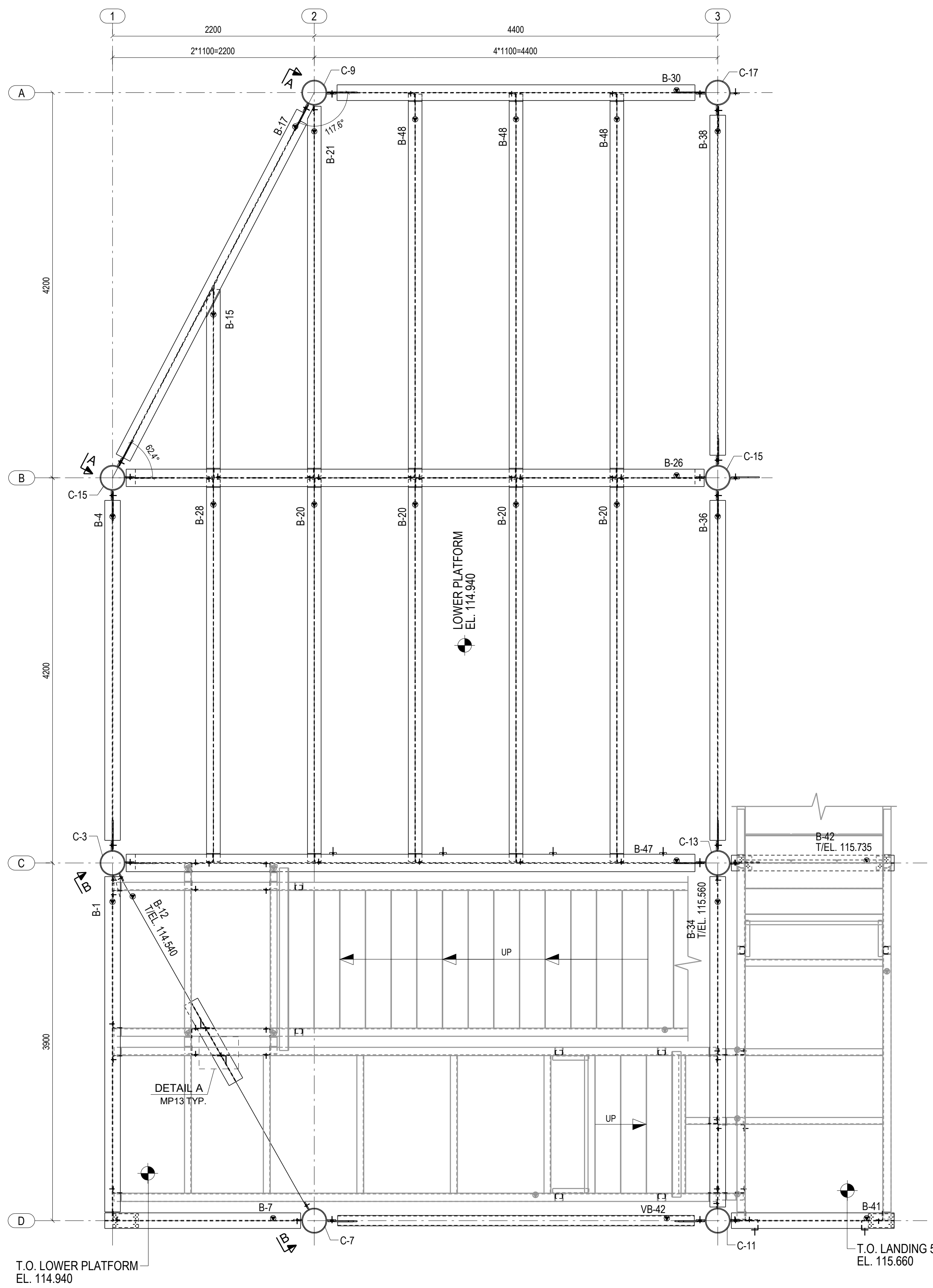
TOWER LOWER PLATFORM FRAMING PLAN
